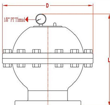
▲ Flange end (AIF) With Pressure Gauge
